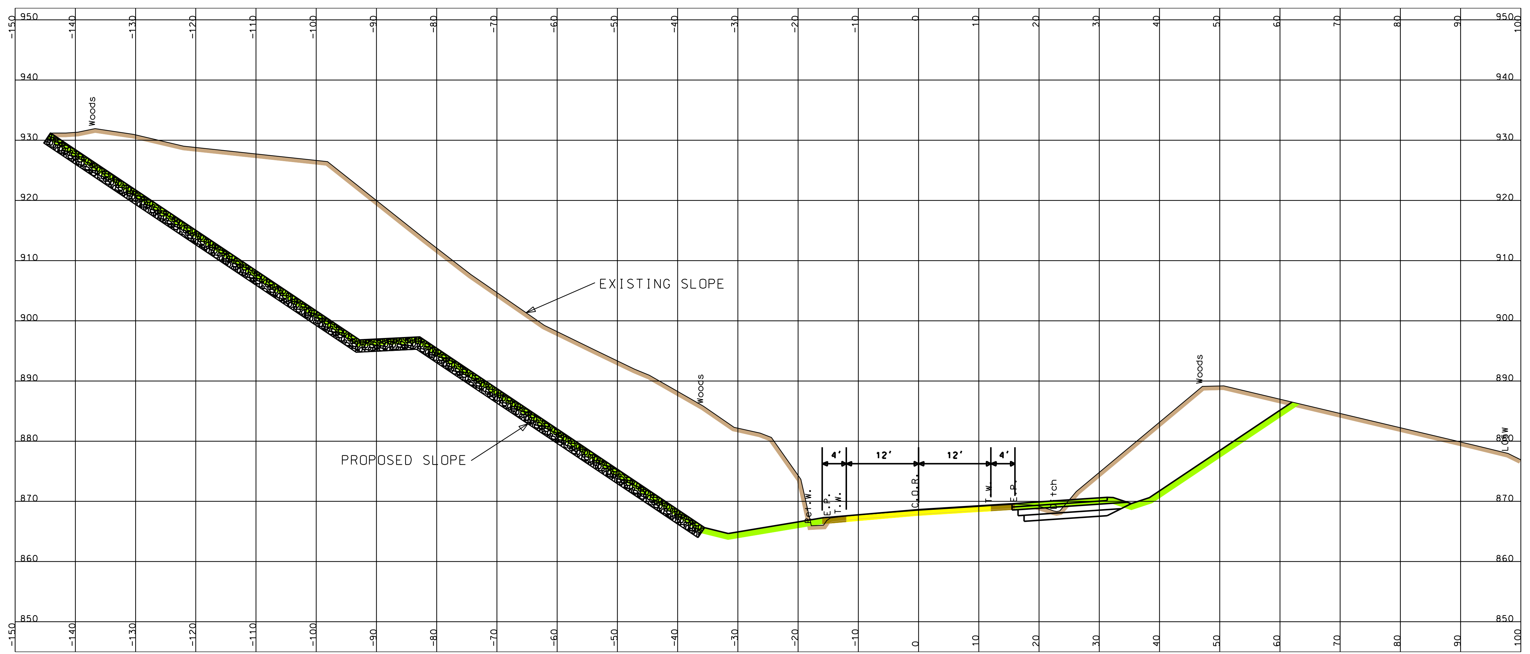
118+50 RETAINING WALL REMOVAL
