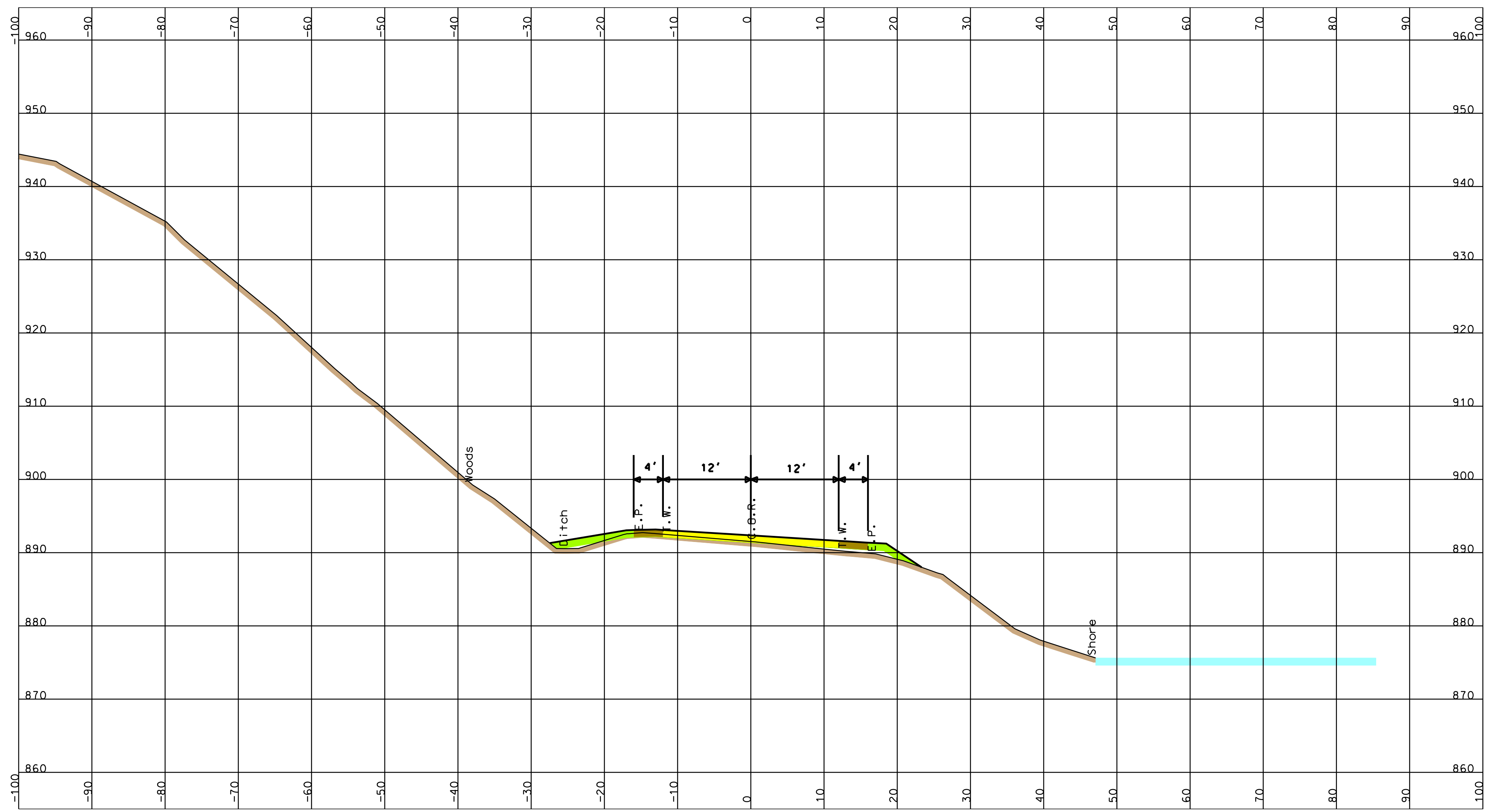
148+00 ROADWAY REHABILITATION
