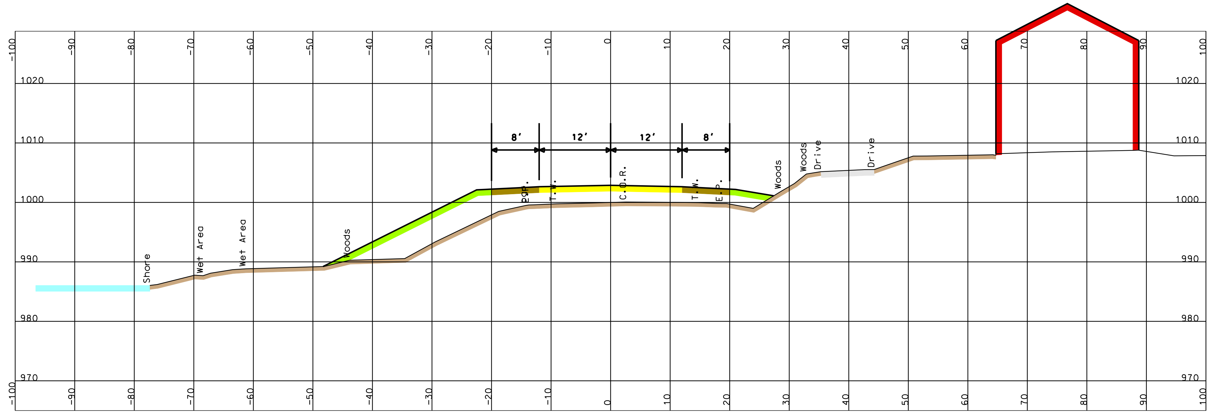
207+80 BRIDGE AREA
