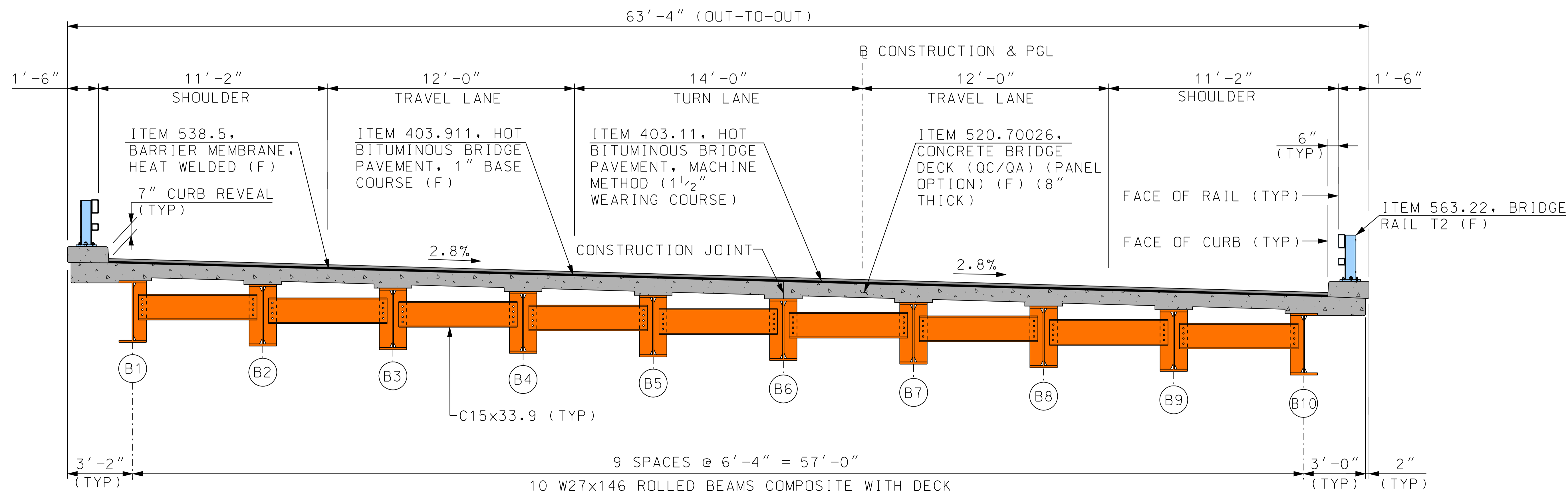
TYPICAL DECK SECTION
