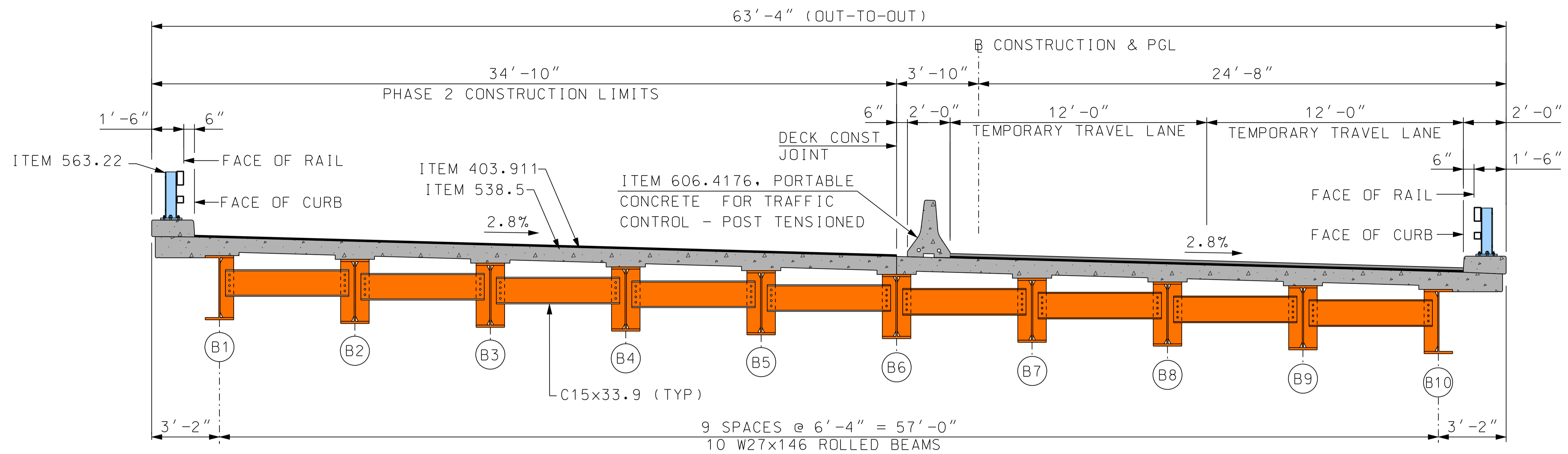
PHASE 2 CONSTRUCTION SECTION
