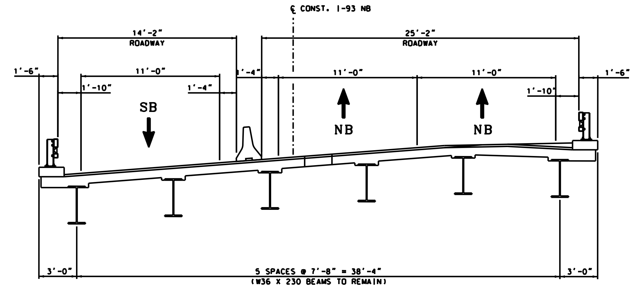
ALTERNATIVE B - WIDEN BOTH BRIDGES STAGE 4
