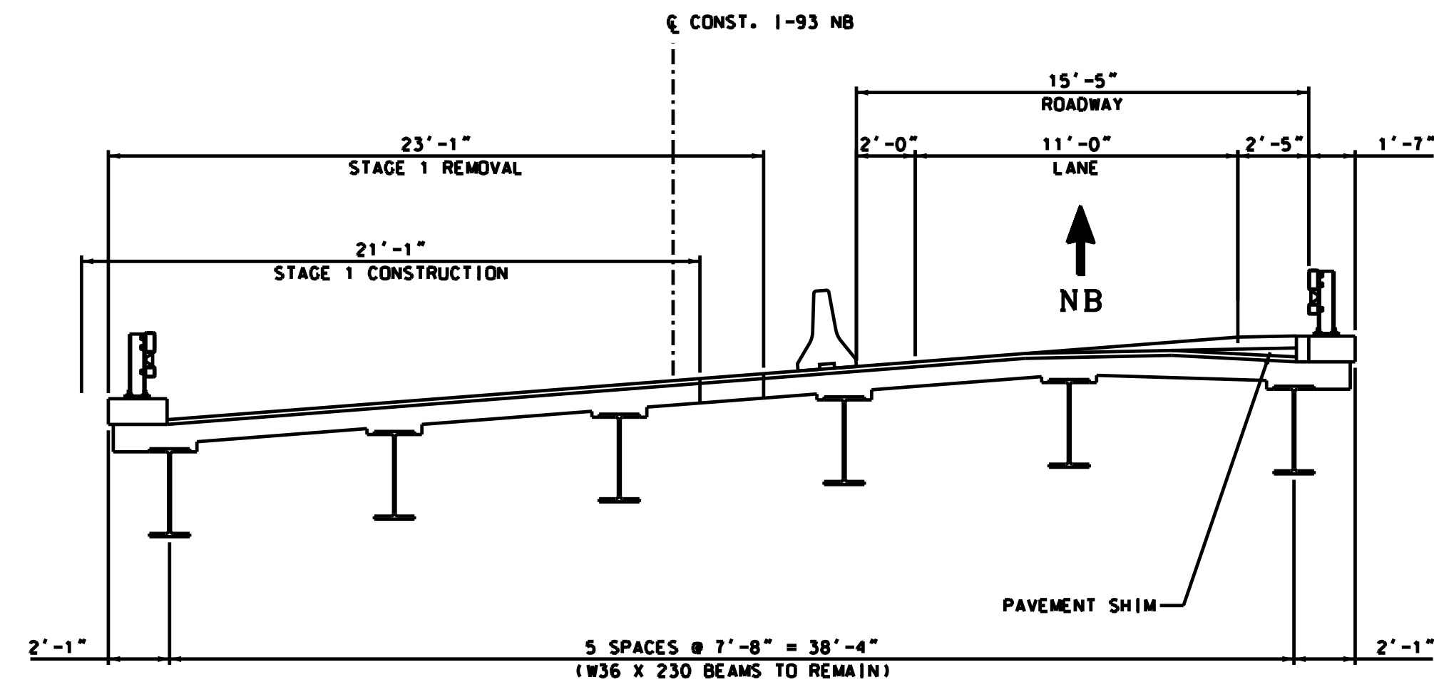
ALTERNATIVE B - WIDEN BOTH BRIDGES STAGE 1
