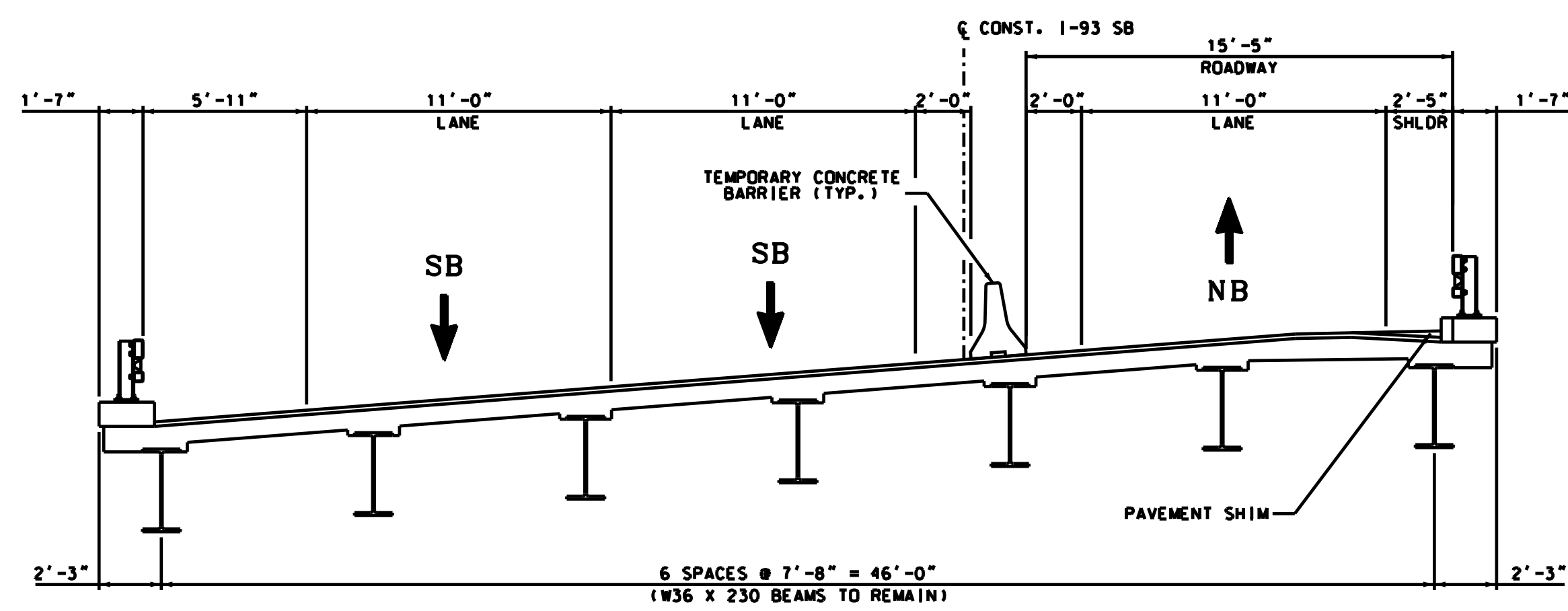
ALTERNATIVE B - WIDEN BOTH BRIDGES STAGE 2
