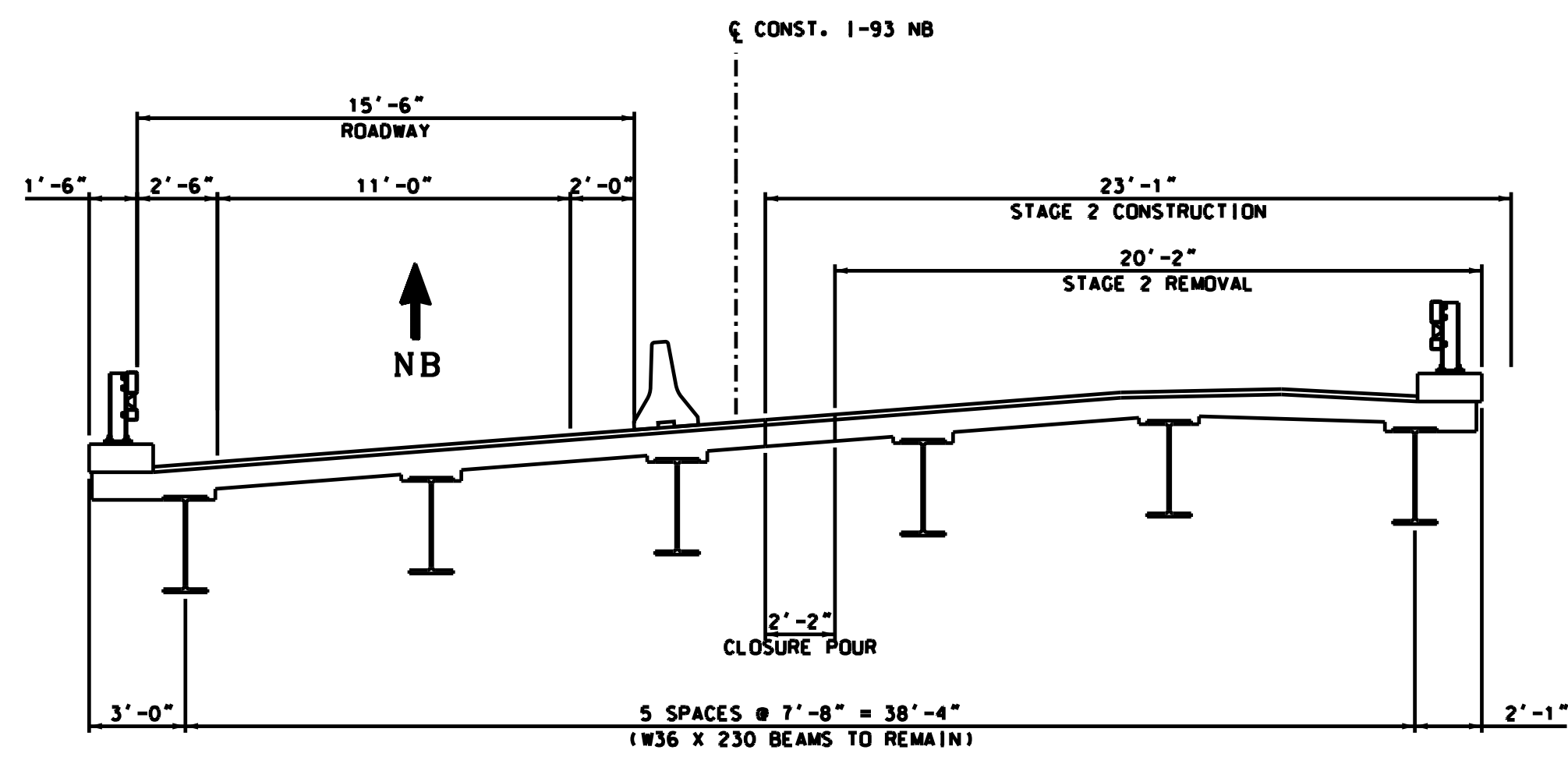
ALTERNATIVE B - WIDEN BOTH BRIDGES STAGE 2
