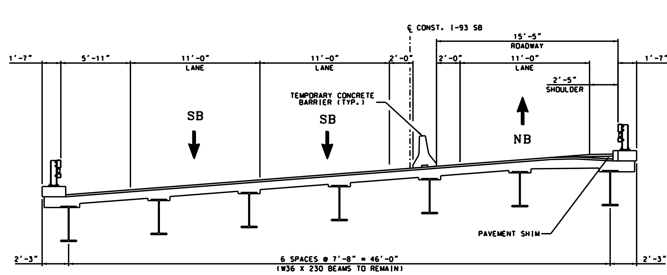
ALTERNATIVE B - WIDEN BOTH BRIDGES STAGE 1
