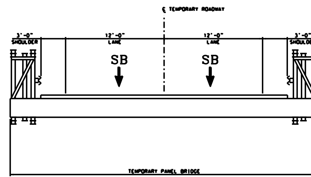
ALTERNATIVE A - TEMPORARY BRIDGE STAGE 2
