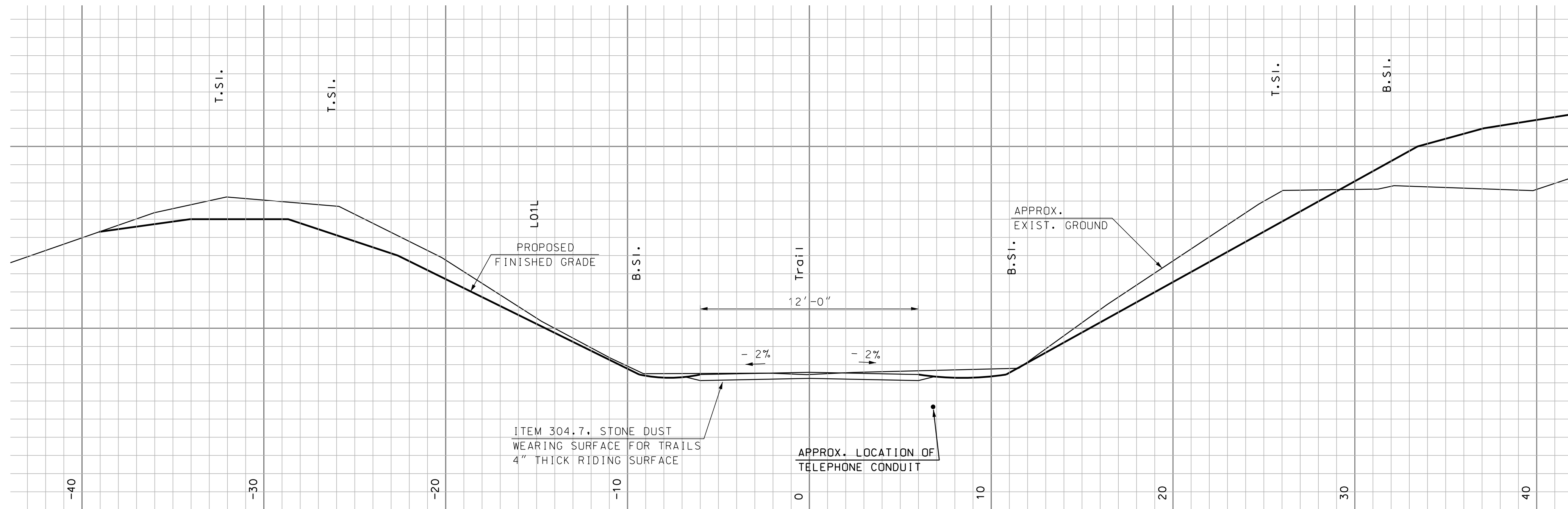
TYPICAL RAIL CORRIDOR SECTION (LOOKING EAST) SCALE: 1/4" = 1'-0"
