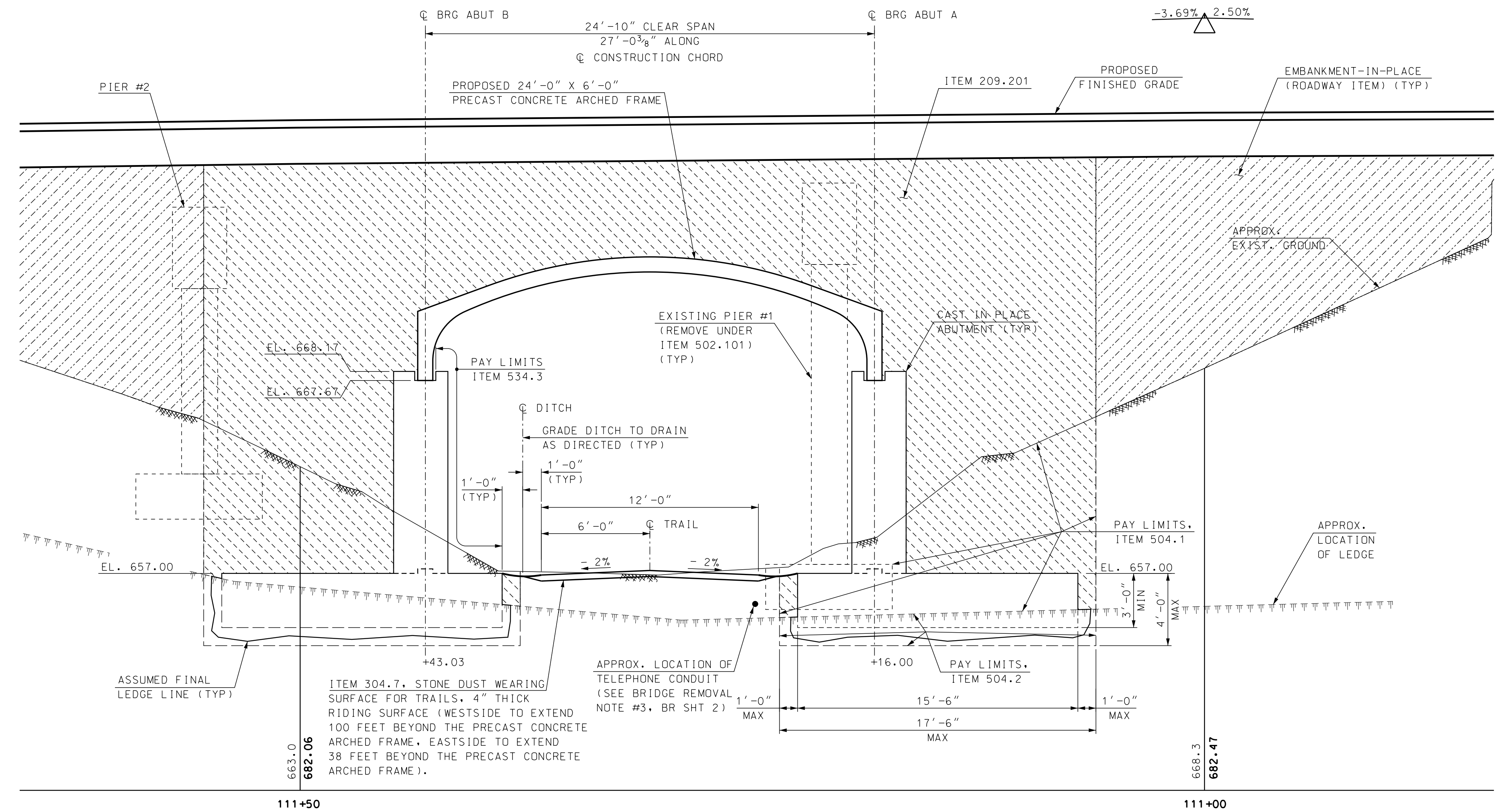
TYPICAL ARCHED FRAME SECTION (LOOKING EAST) SCALE: 1/4" = 1'-0"
